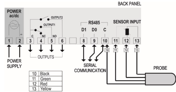
Figure 2 – Electrical connections
