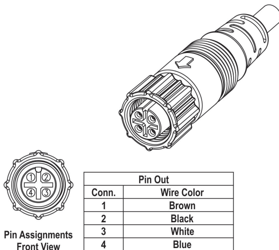
Fig. 6 – Connecting pins for M12 cable mounting
