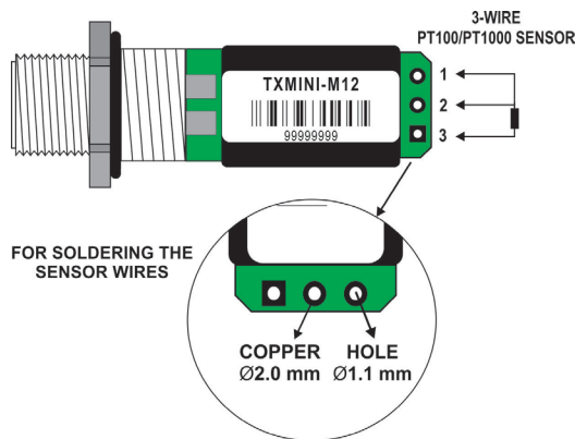
Fig. 5 – Input 3-wire Pt100 / Pt1000
