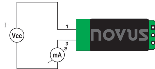
Fig. 4 – TxMini-M12 / TxMini Connection Diagram
