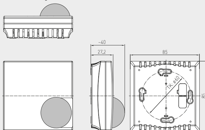
Dimensional drawing
