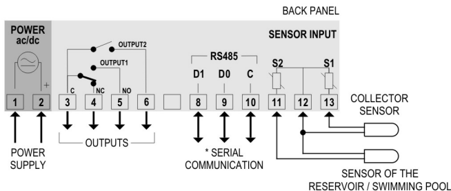
Fig. 1 – N322S terminals
