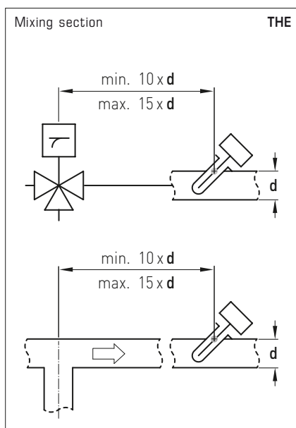
Installation scheme
