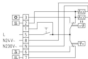
Connecting diagram
