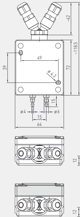
Dimensional drawing
