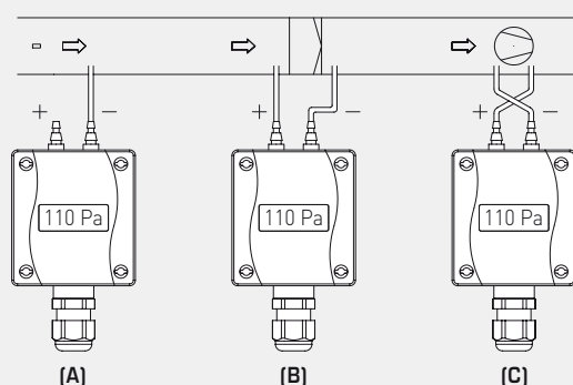
Mounting diagram
