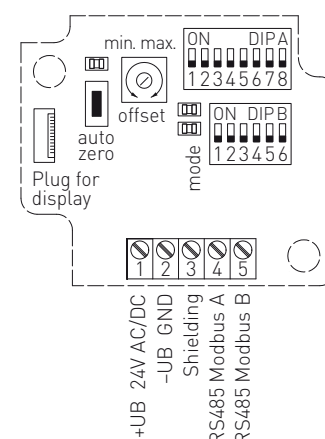
Schematic diagram PREMASGARD® 121x-Modbus
