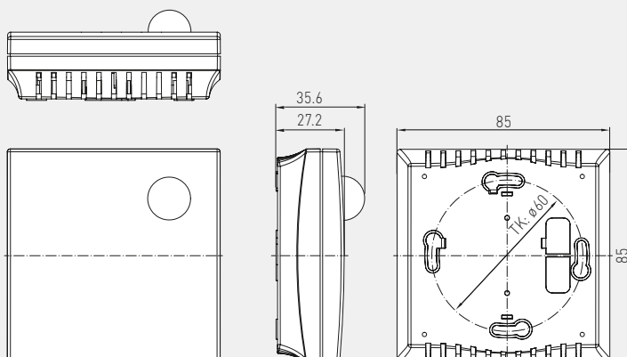
Dimensional drawing
