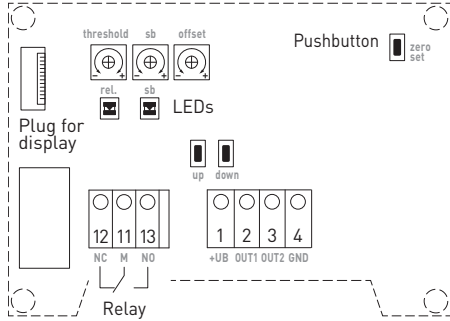
Connecting diagram
