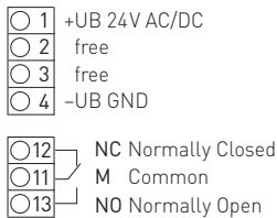
Connecting diagram
