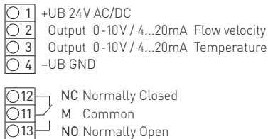
Connecting diagram
