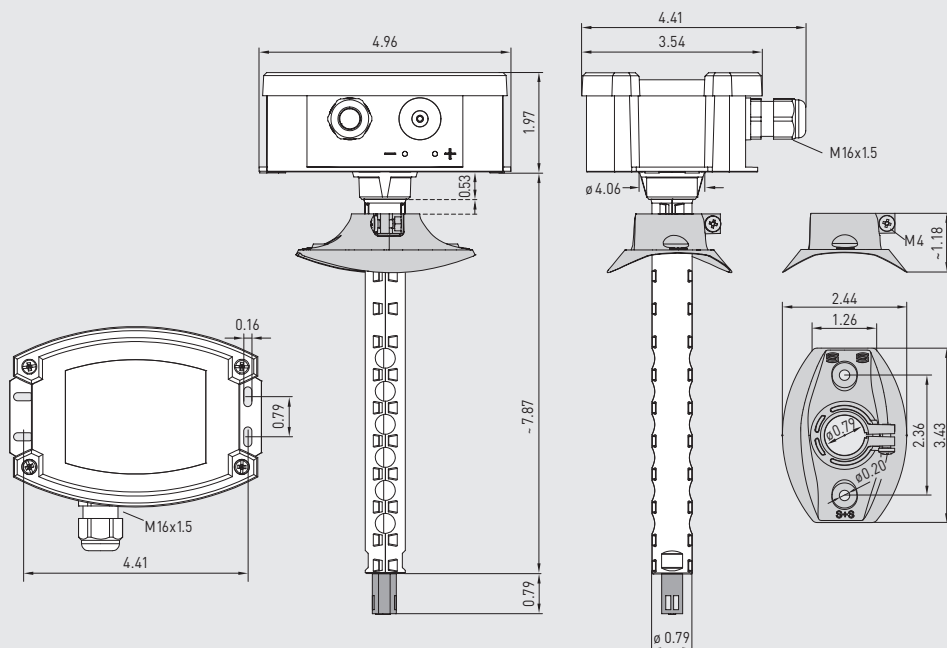
Dimensional drawing [inch]
